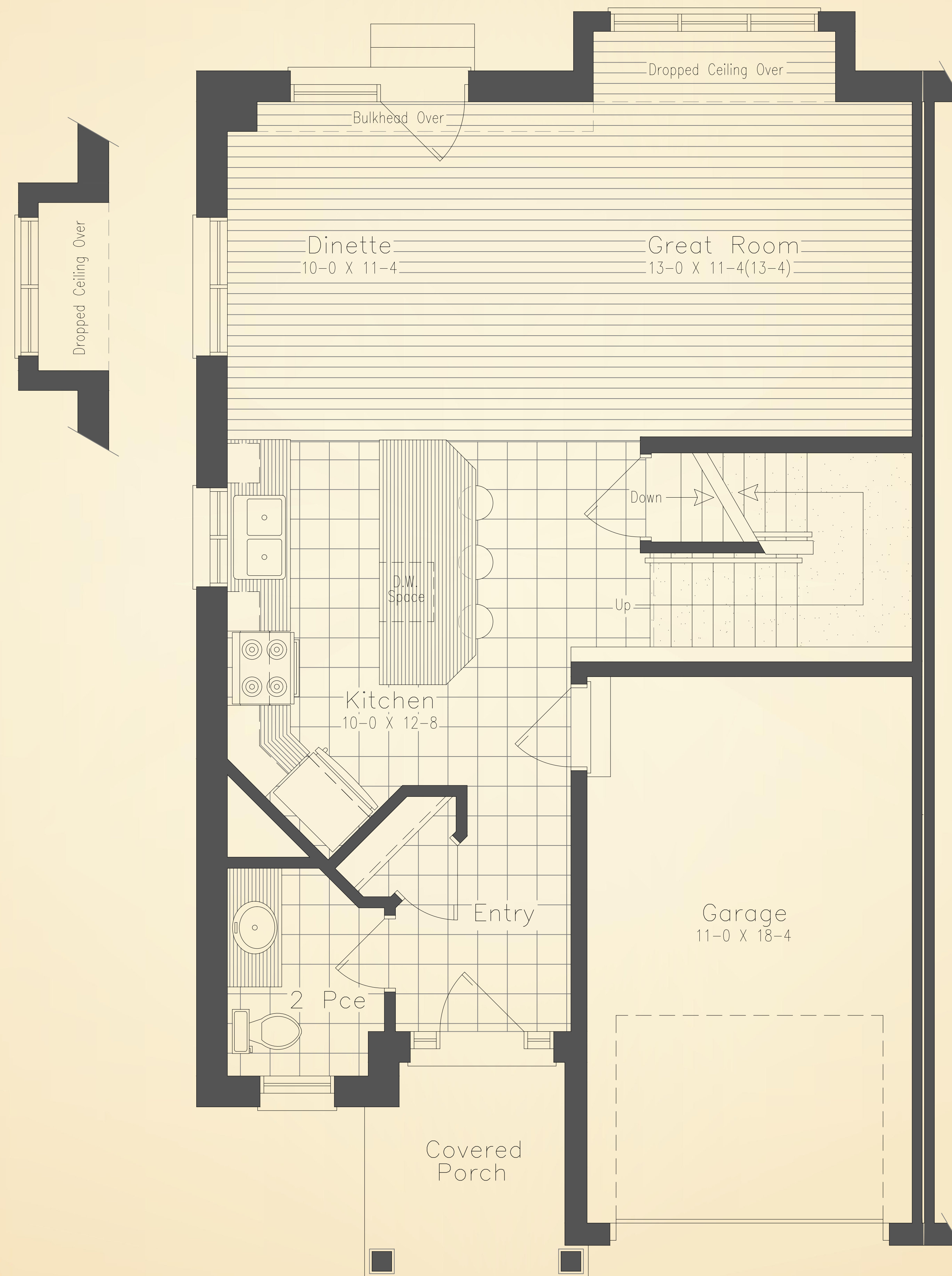
Main Floor Layout (End Unit area - 706 s.f.)
